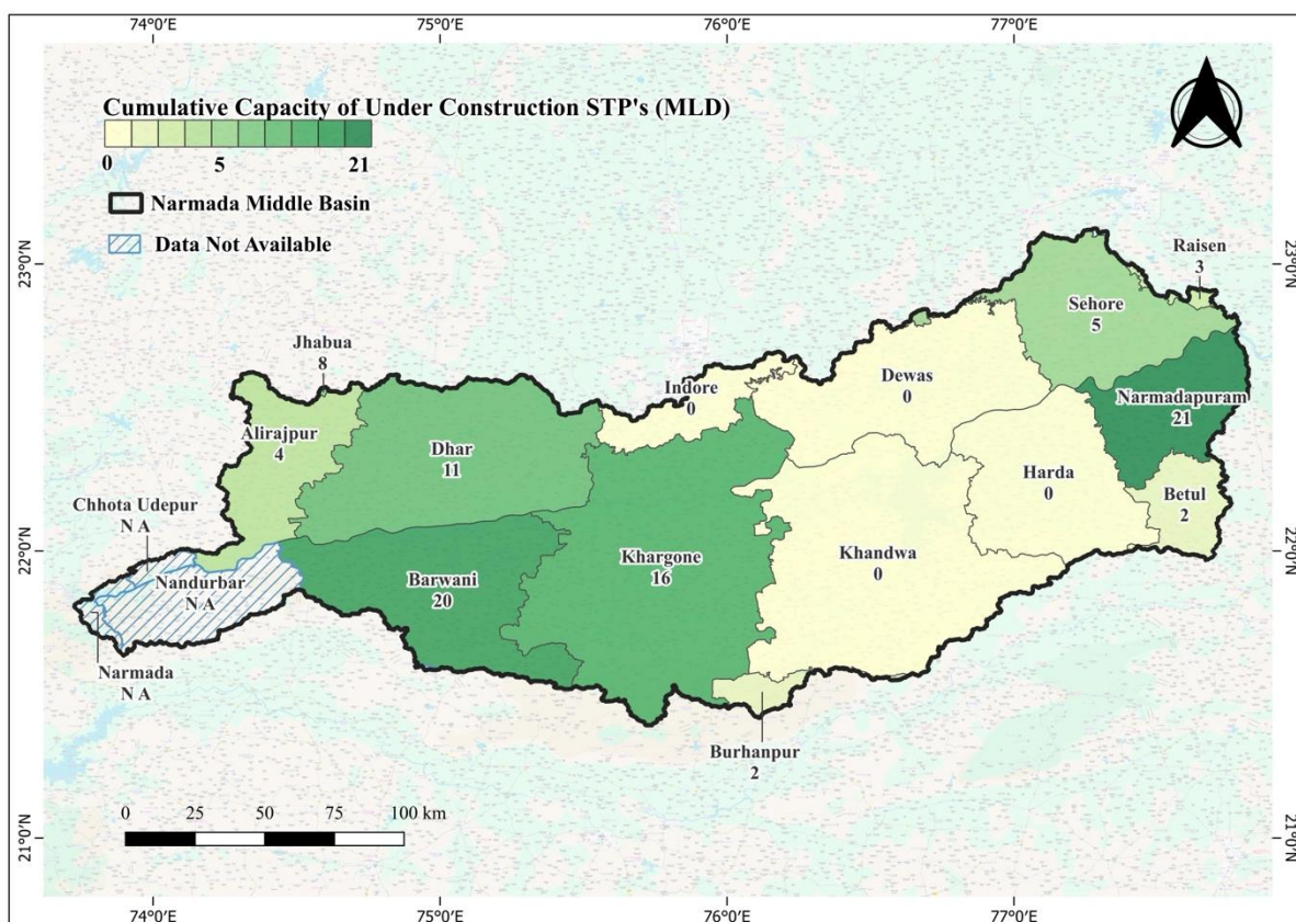
Figure 16 District-wise cumulative capacity (MLD) of under-construction STPs in Narmada Middle Basin
